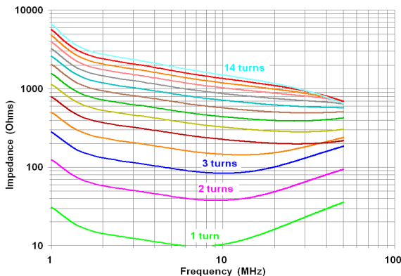
#77 Impedance
