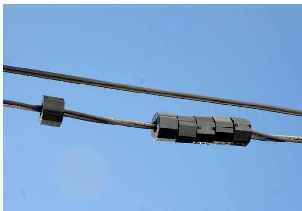
Fig 31 – Chokes on a Power Line
