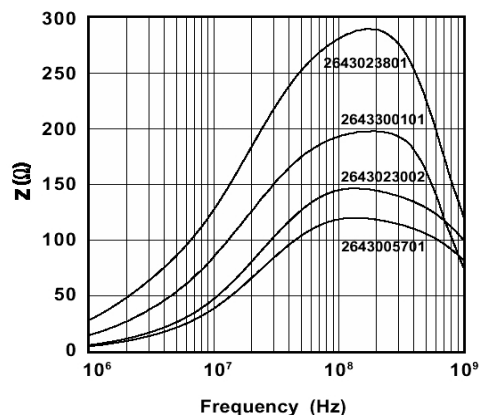
Fig 9 – Small cores of different lengths
