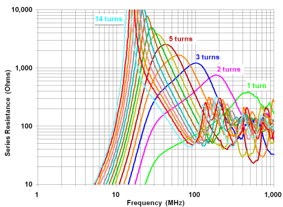
#61 Resistance VHF
