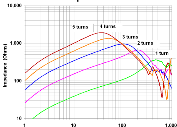
#43 Impedance VHF
