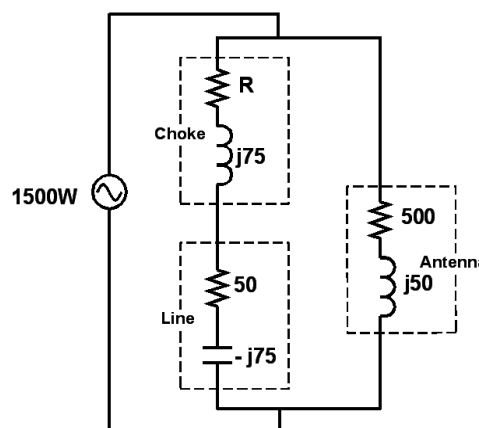
Fig 36 – A Common Mode Choke Applied to a Transmission Line
